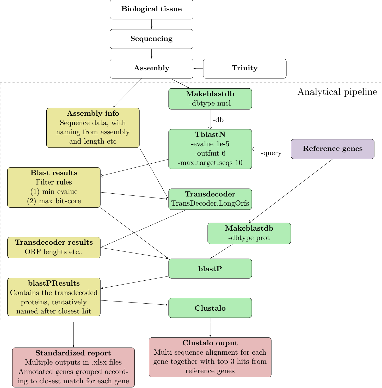
Figure 0.1: Work flow for automated annotation of genes. Different colors means; yellow: results that are integrated to a database within R; green: external softwares that are called from within R; purple are information that needs to be provided and curated; red are the reports for the end users; and white are steps that are not encompassed by the pipeline.
